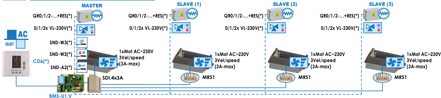
Fig.4 MASTER-SLAVE (Open-space System)
