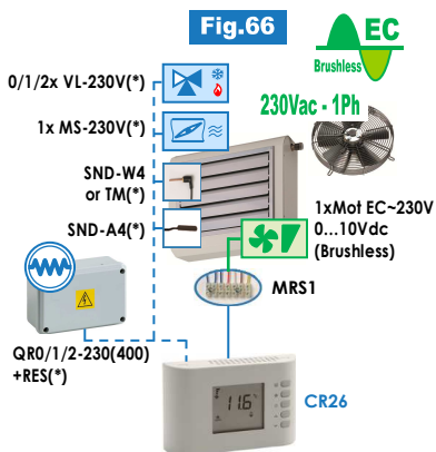
(*) Accessori/es: SND-A4, SND-W4, TM, VL-230V, QRO/1/2-230(400)+RES, MS-230V
