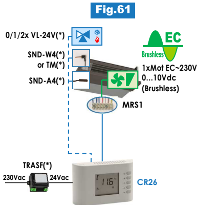
(*) Accessori/es: SND-A4, SND-W4, TM, VL-24V
