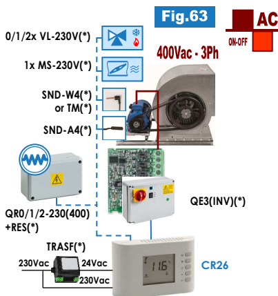
(*) Accessori/es: TRASF, QE3(INV), SND-A4, SND-W4, TM, VL-230V, QRO/1/2-230(400)+RES, MS-230V
