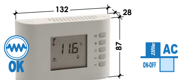
CR25 - FAN: MOT_AC~230V - Valvole-Valves: ON/OFF, PWM, 3-Point
