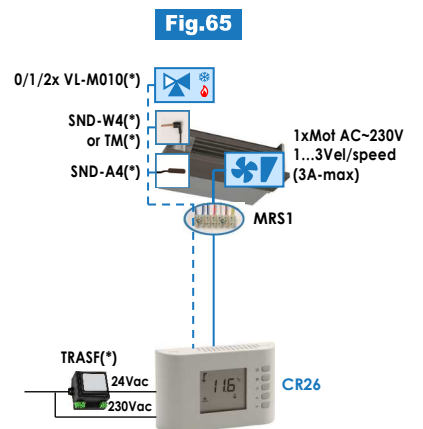
(*) Accessori/es: TRASF, SND-A4, SND-W4, TM, VL-M010
