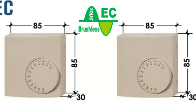
TR11 • 0...10Vdc • Range 6-30°C TR12 • 0...10Vdc • Range 20-70°C
