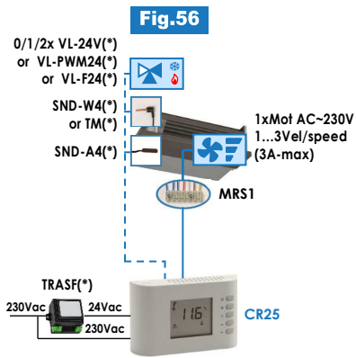
(*) Accessori/es: TRASF, SND-A4, SND-W4, TM, VL...
