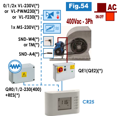
(*) Accessori/es: QE1(QE2), SND-A4, SND-W4, TM, VL..., QR0/1/2-230(400)+RES, MS-230V
