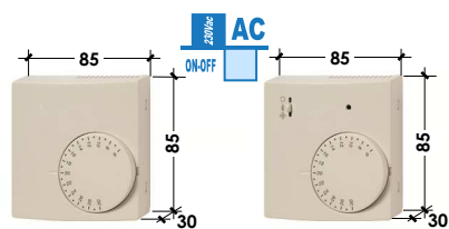
TR0 • ON/OFF • Solo risc., Heating only • Range 6-30°C TR1 • ON/OFF • Range 6-30°C
