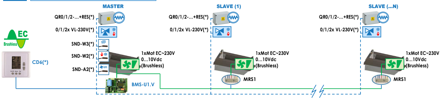
Fig.5 MASTER-SLAVE (Open-space System)
